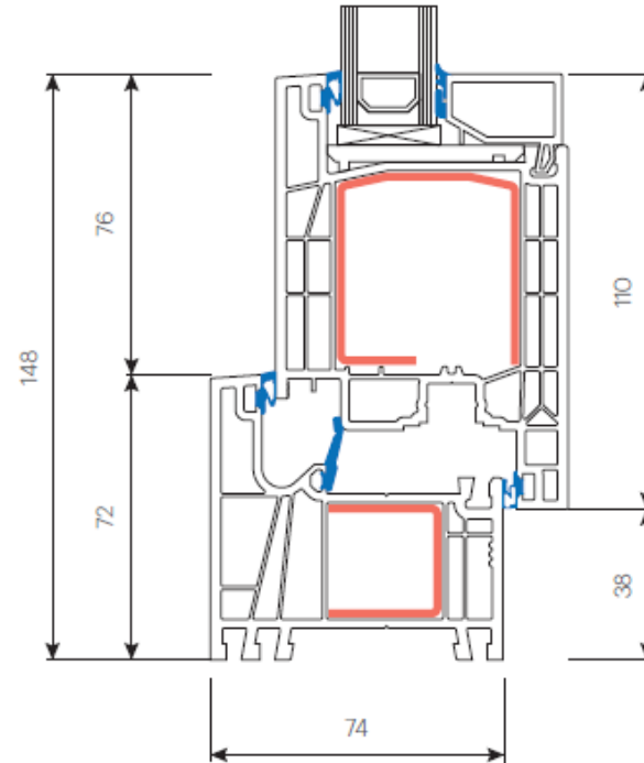
Internal opening way (7001+7082)
