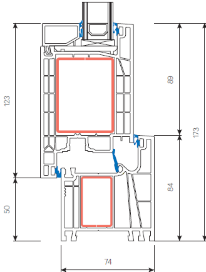
Entry doors (7005 +7088)
