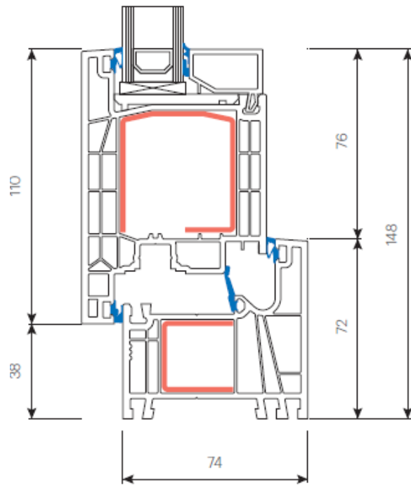
External opening way (7001+7084)
